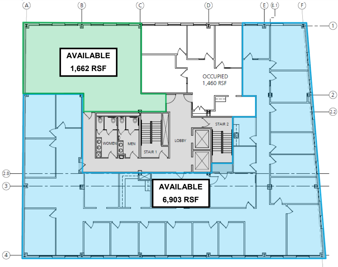
2ND FLOOR PLAN SCALE: 1/16" = 1'-0" 4/15/2022
